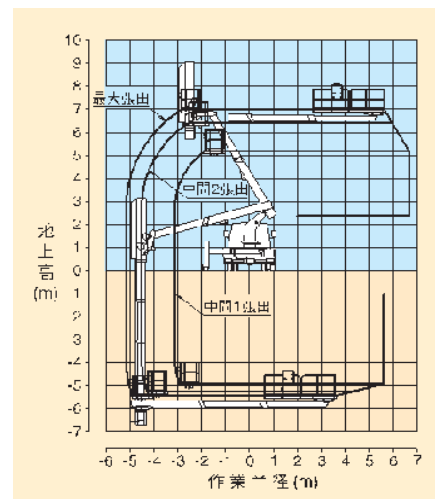
図2 橋梁点検車(BT-200)作業範囲
